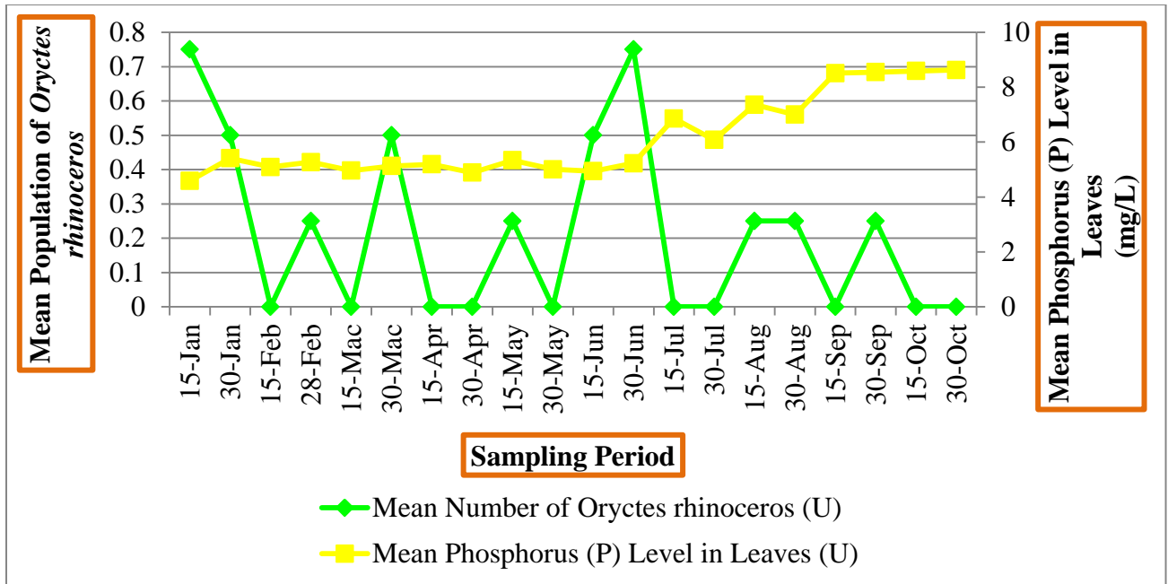
Fig 3: Interaction Between Mean Population of Oryctes rhinoceros against Mean Phosphorus (P) Level in Oil Palm's Leaves at Untreated area.
